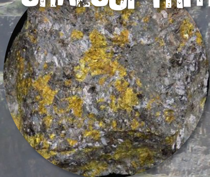
SPHALERITE & CHALCOPYRITE
